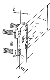
(1) Die-cast aluminium
