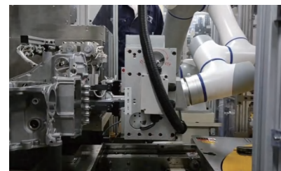
Gearbox Screw Locking
