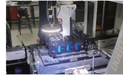
Energy Storage Battery Screw Locking
