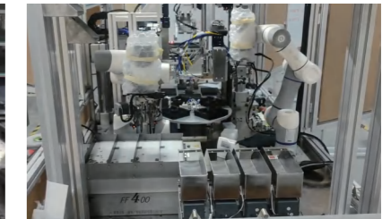
Electronic Component Sorting
